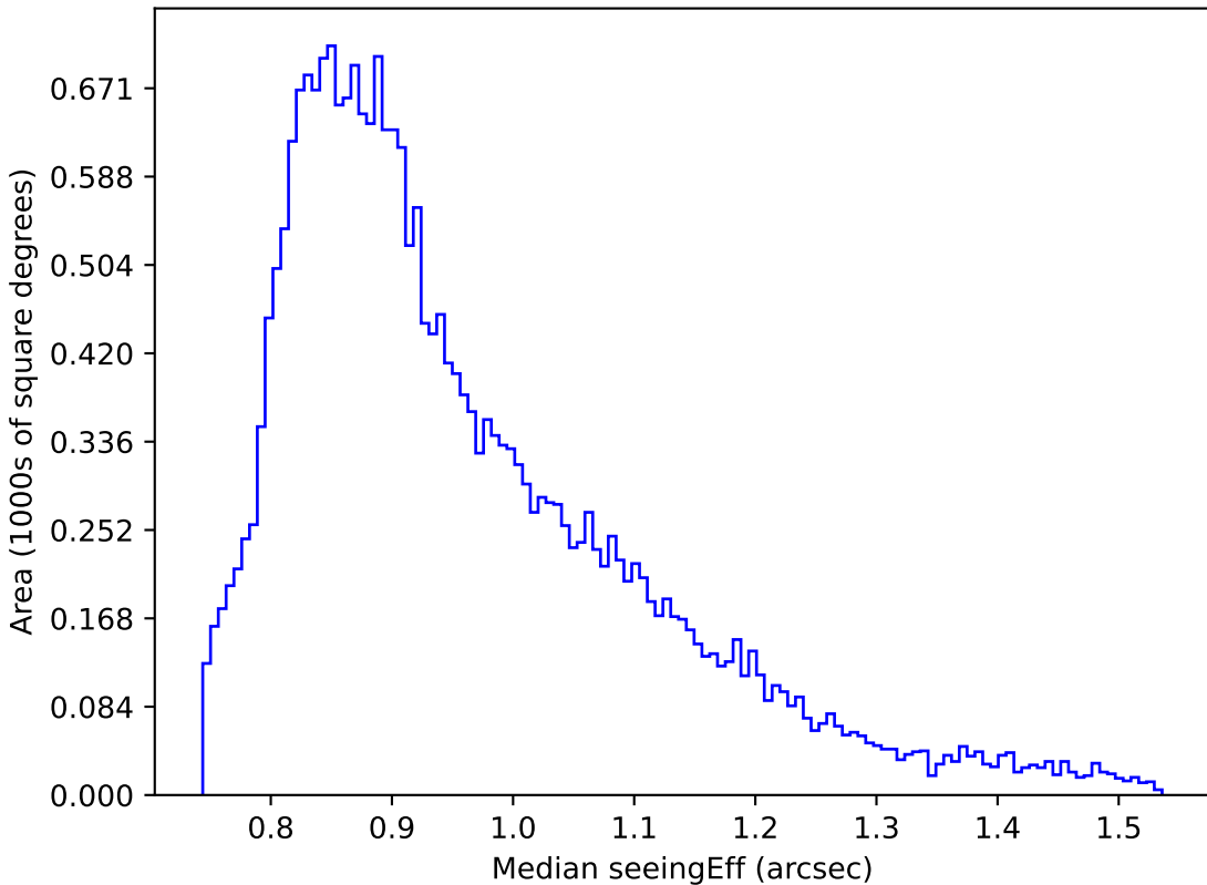
baseline_v2.1_10yrs Yr 1 r band: Median seeingEff
