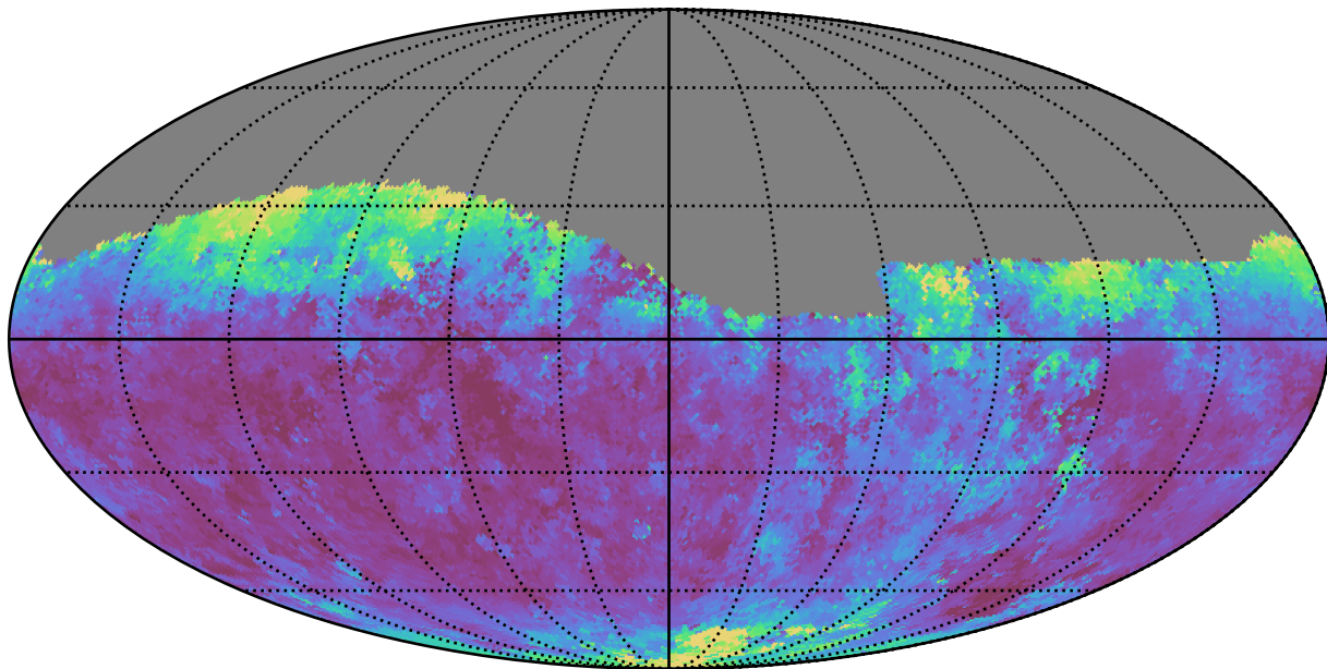
baseline_v2.1_10yrs Yr 1 i band: Median seeingEff
