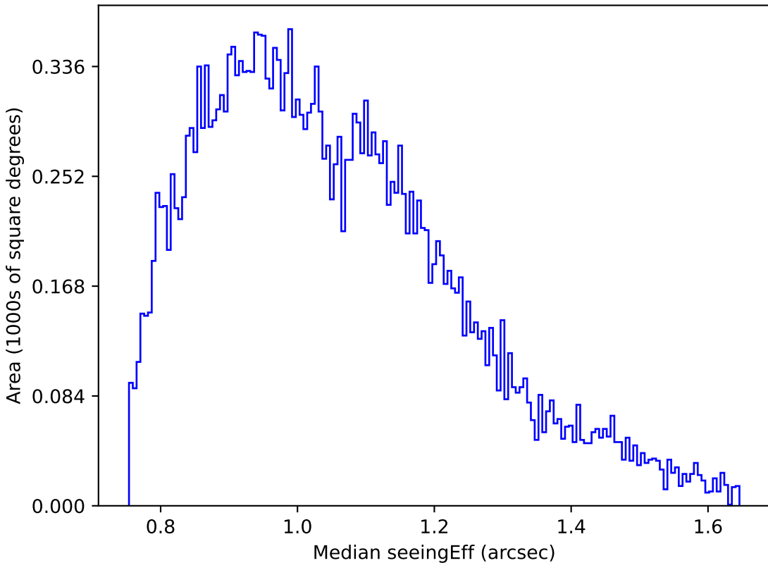
baseline_v2.1_10yrs Yr 1 g band: Median seeingEff
