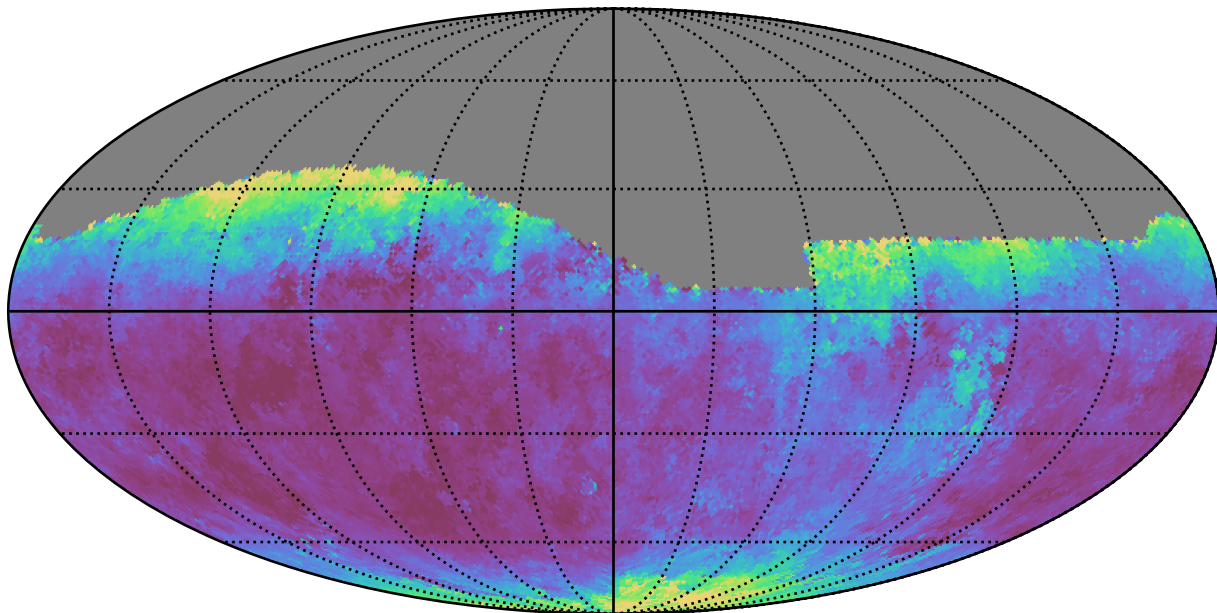
baseline_v2.1_10yrs Yr 1 all bands: Median seeingEff
