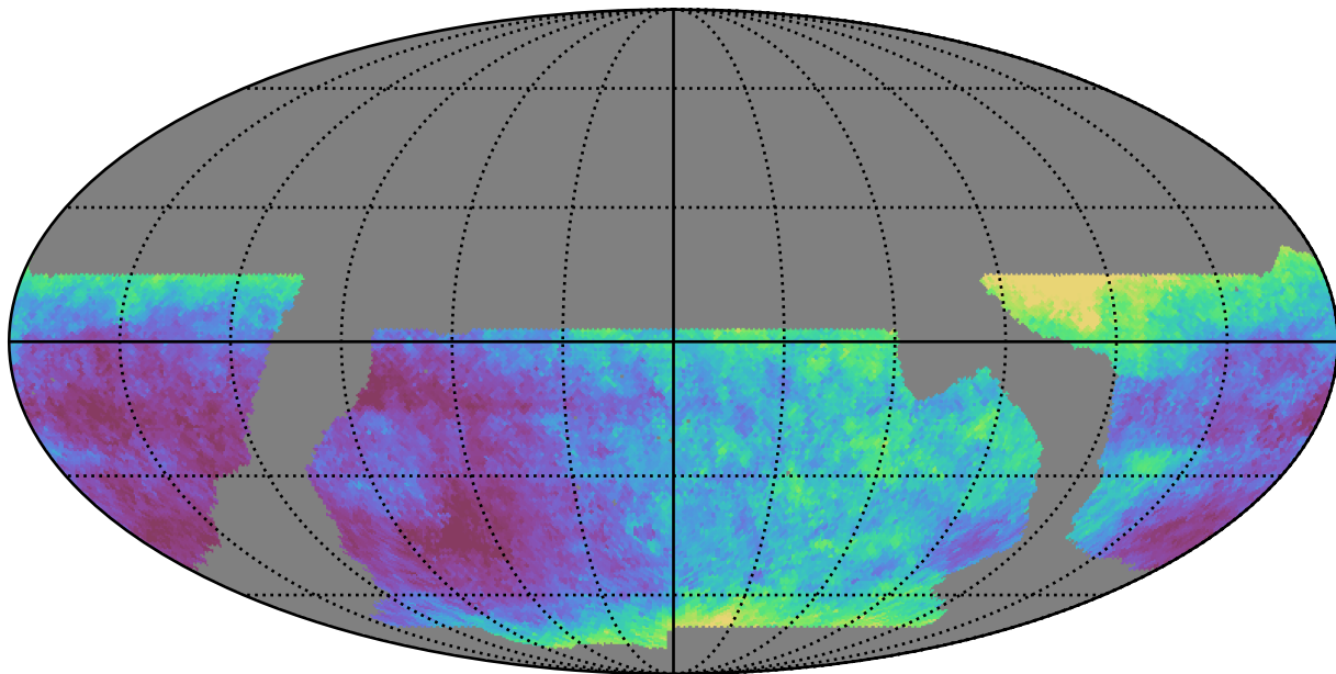
baseline_v2.1_10yrs WFD z band: Median seeingEff
