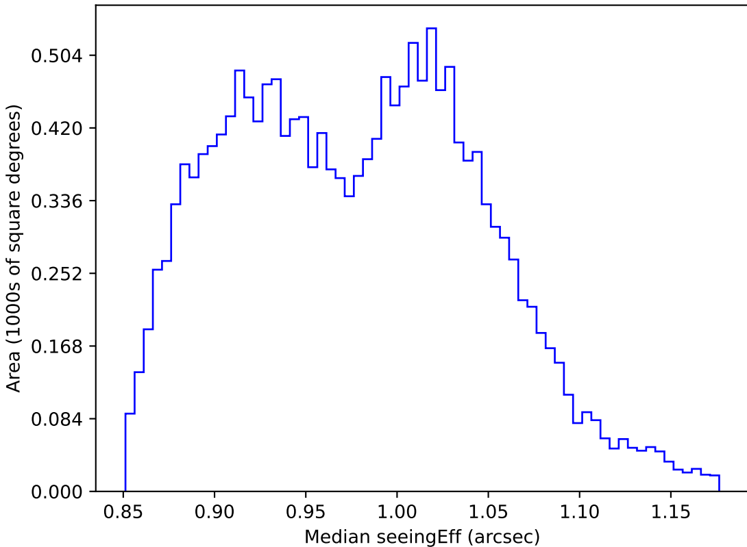
baseline_v2.1_10yrs WFD z band: Median seeingEff
