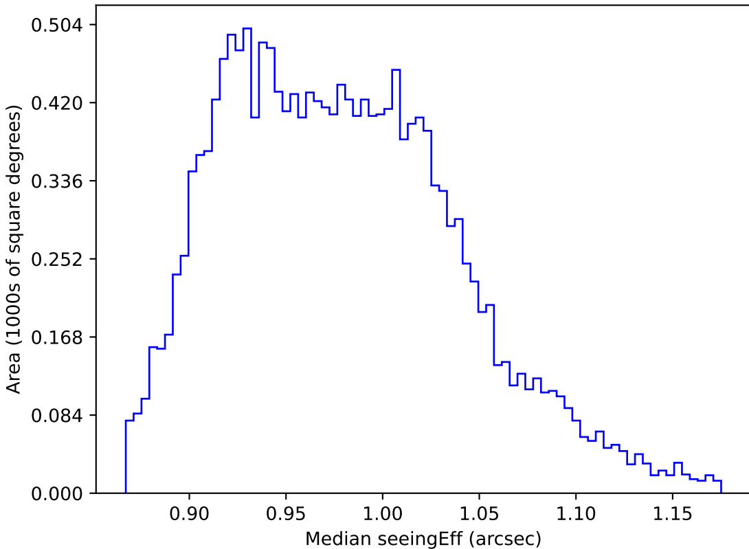
baseline_v2.1_10yrs WFD y band: Median seeingEff
