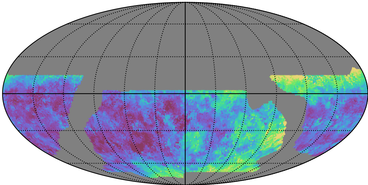
baseline_v2.1_10yrs WFD u band: Median seeingEff
