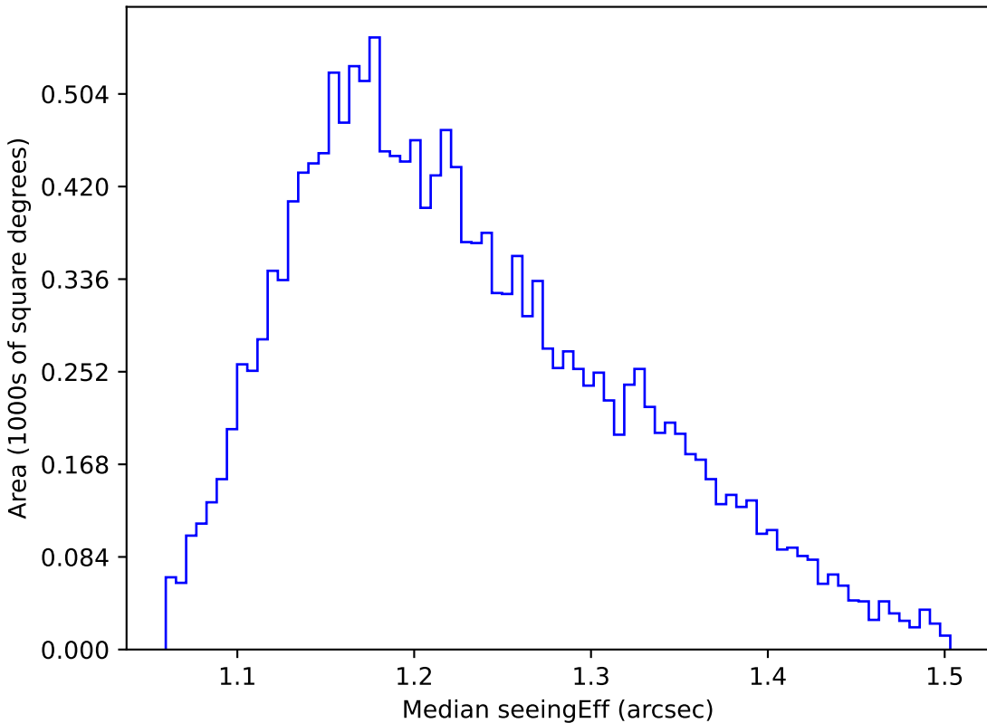
baseline_v2.1_10yrs WFD u band: Median seeingEff
