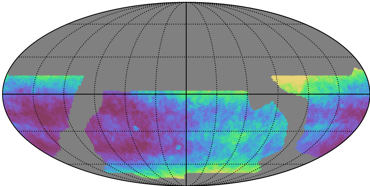
baseline_v2.1_10yrs WFD r band: Median seeingEff
