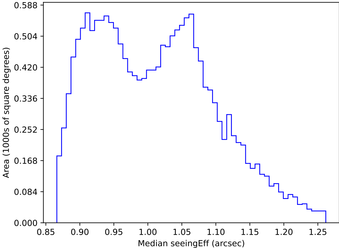
baseline_v2.1_10yrs WFD r band: Median seeingEff
