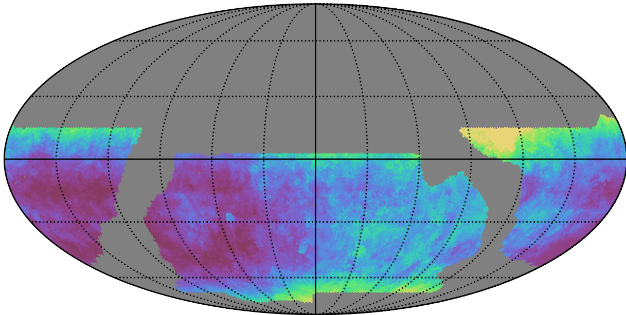
baseline_v2.1_10yrs WFD i band: Median seeingEff
