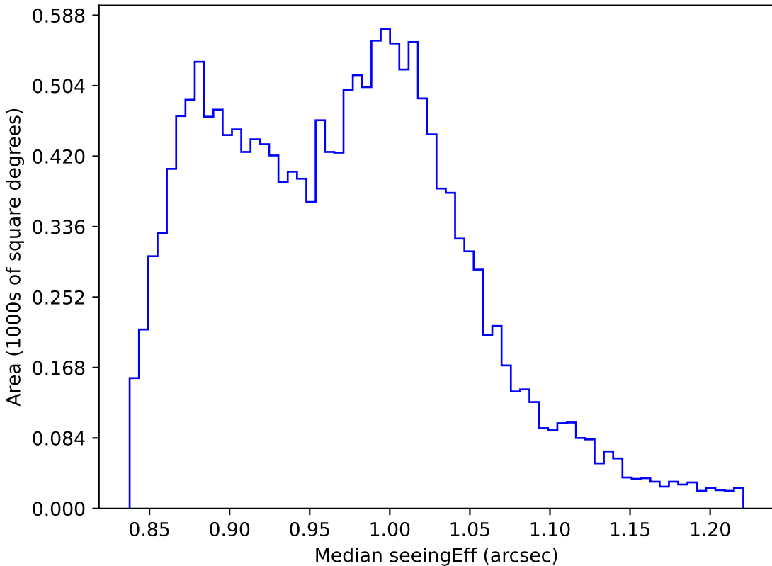
baseline_v2.1_10yrs WFD i band: Median seeingEff
