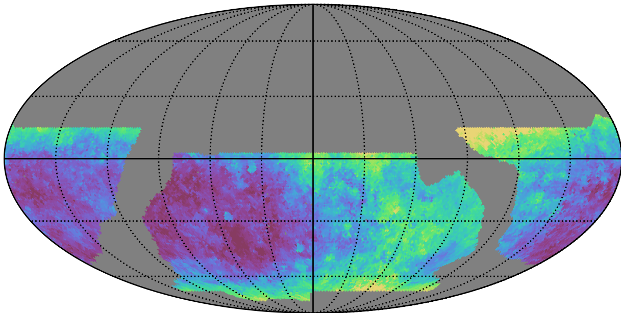
baseline_v2.1_10yrs WFD g band: Median seeingEff
