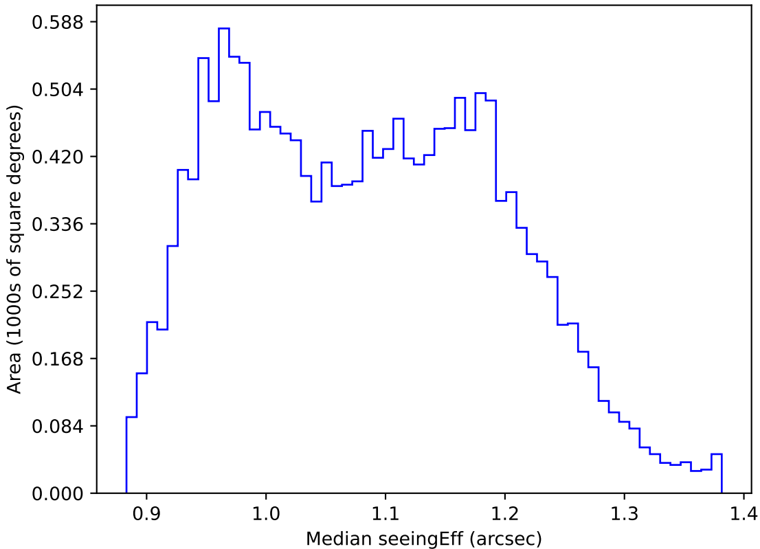
baseline_v2.1_10yrs WFD g band: Median seeingEff
