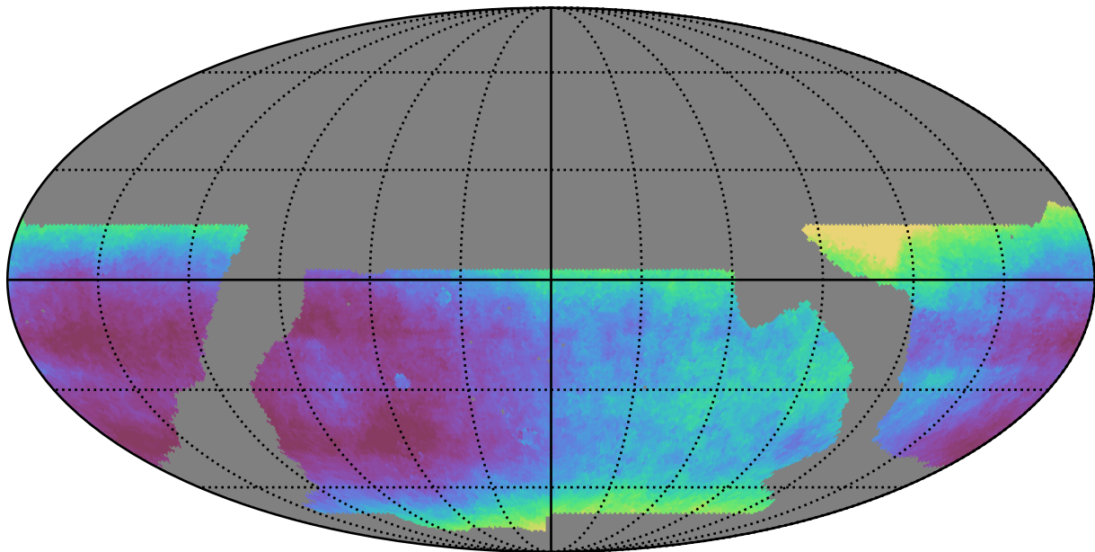
baseline_v2.1_10yrs WFD all bands: Median seeingEff
