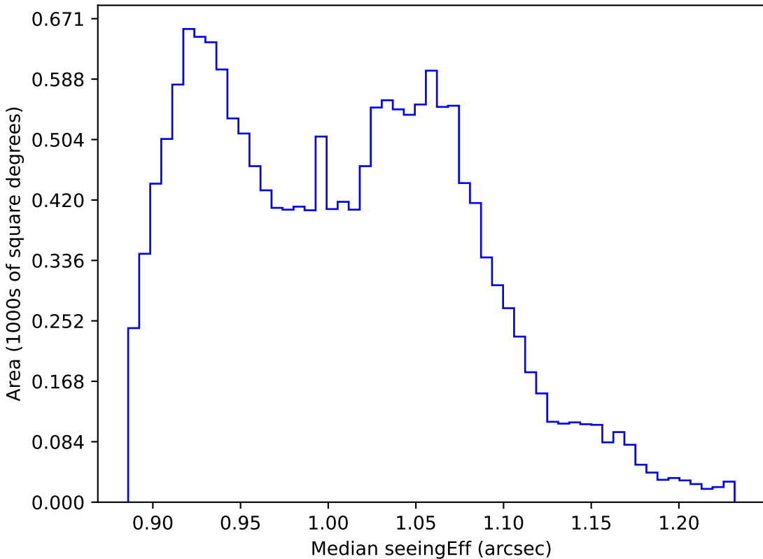
baseline_v2.1_10yrs WFD all bands: Median seeingEff
