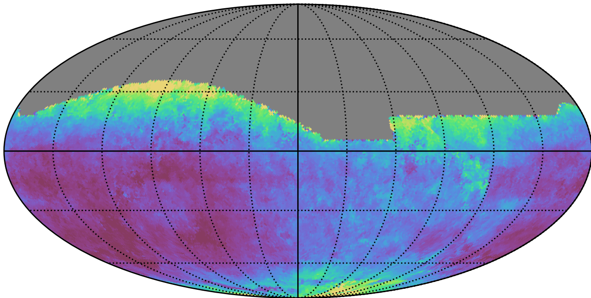
baseline_v2.1_10yrs All sky z band: Median seeingEff
