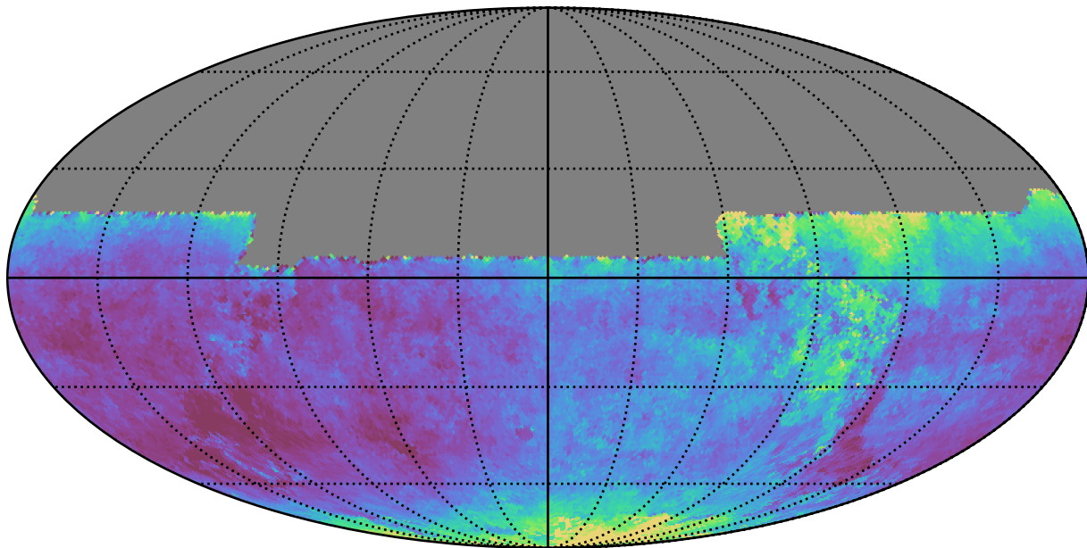
baseline_v2.1_10yrs All sky y band: Median seeingEff
