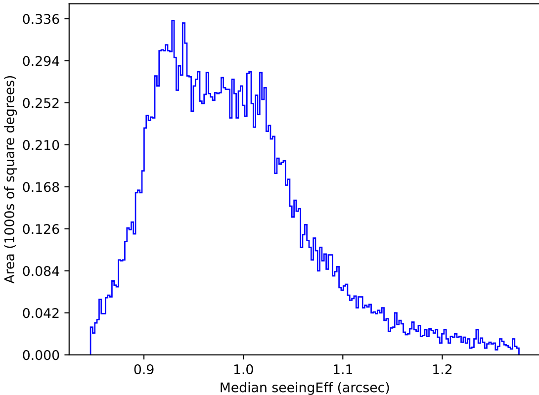
baseline_v2.1_10yrs All sky y band: Median seeingEff
