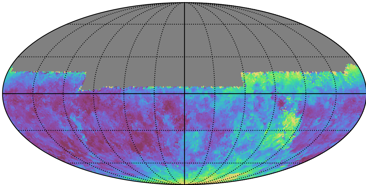
baseline_v2.1_10yrs All sky u band: Median seeingEff
