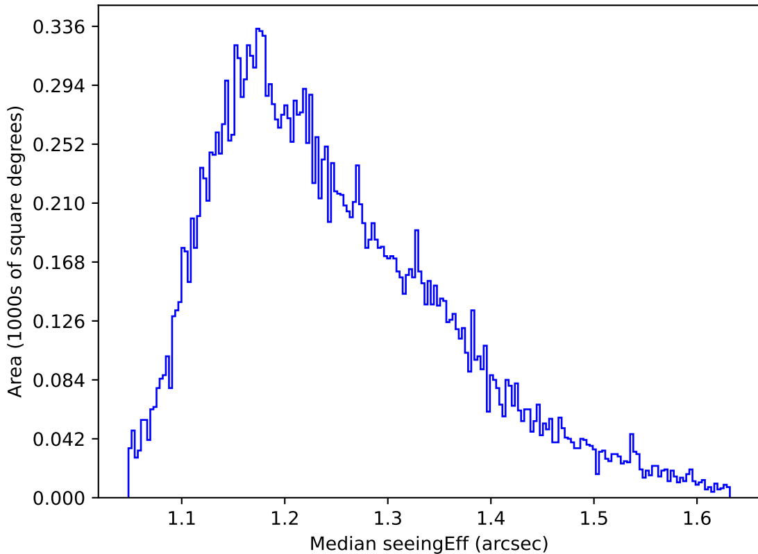
baseline_v2.1_10yrs All sky u band: Median seeingEff
