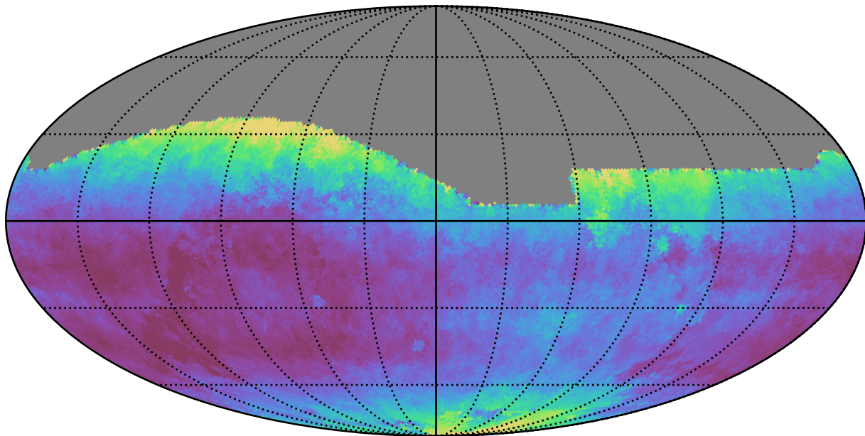
baseline_v2.1_10yrs All sky r band: Median seeingEff
