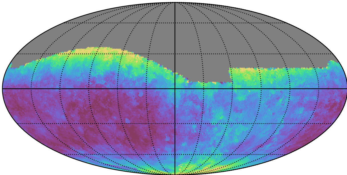
baseline_v2.1_10yrs All sky g band: Median seeingEff
