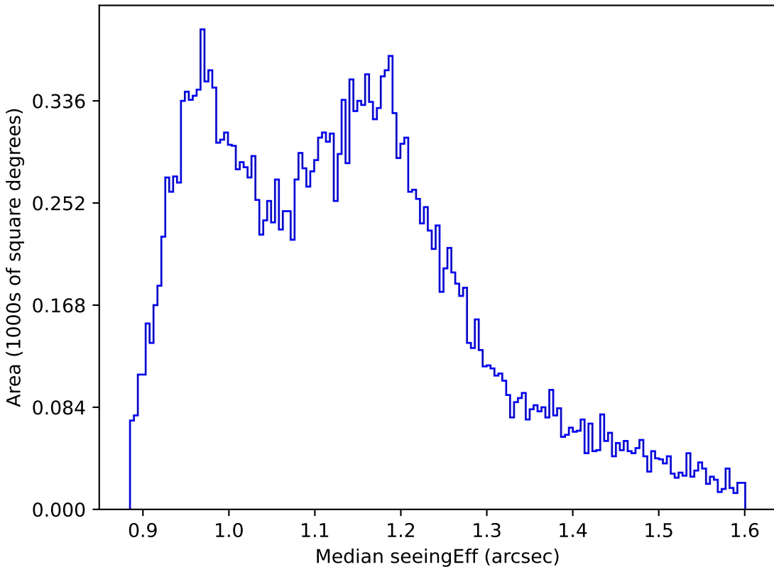
baseline_v2.1_10yrs All sky g band: Median seeingEff
