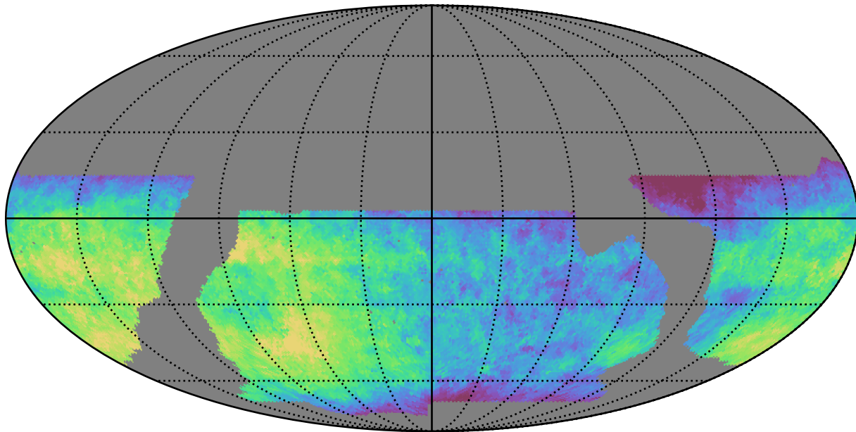
baseline_v2.1_10yrs WFD z band: Median saturation_mag
