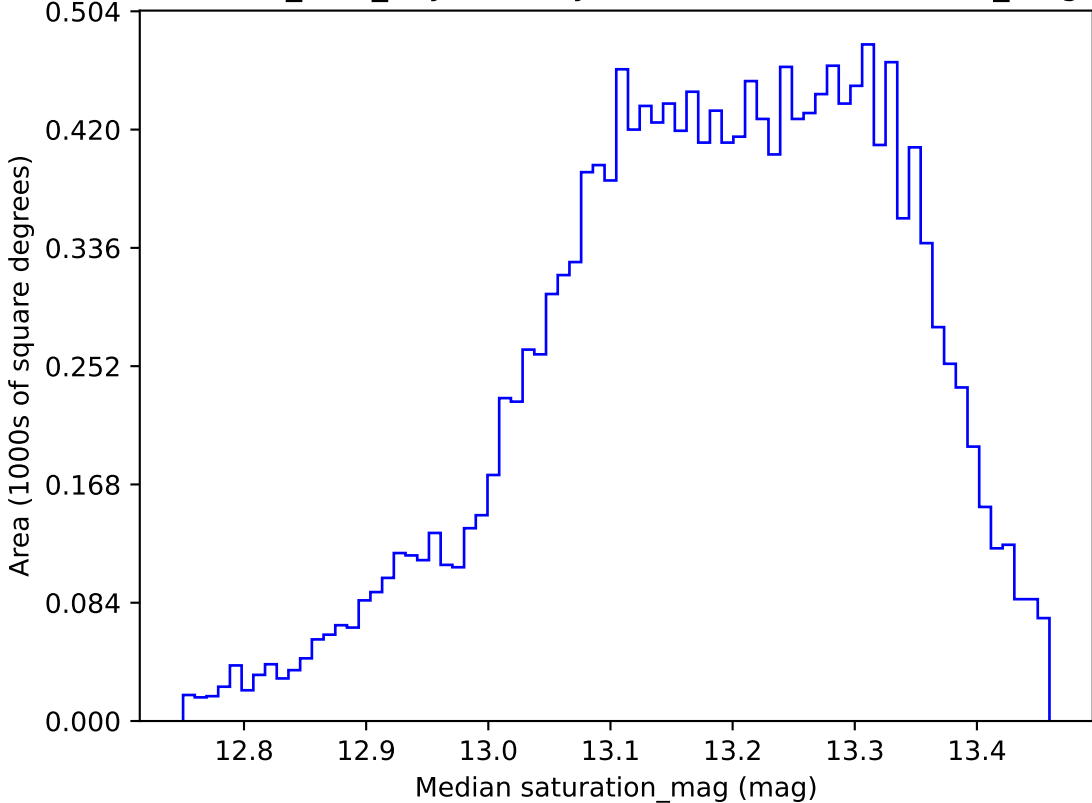
baseline_v2.1_10yrs WFD y band: Median saturation_mag
