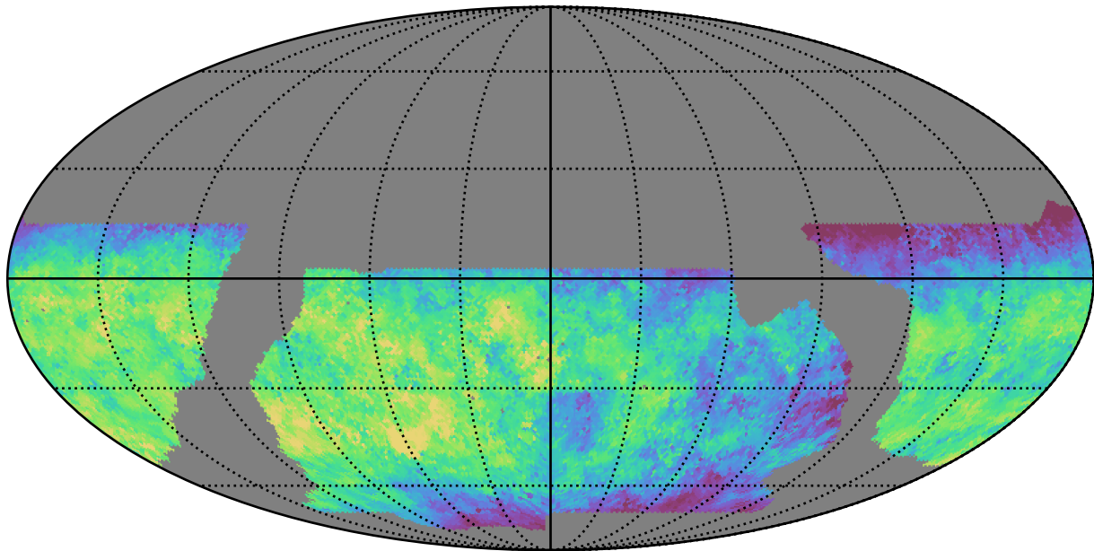
baseline_v2.1_10yrs WFD u band: Median saturation_mag
