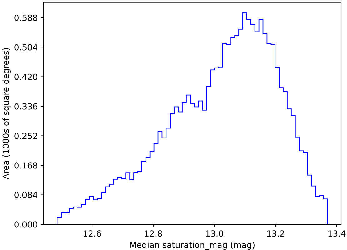
baseline_v2.1_10yrs WFD u band: Median saturation_mag
