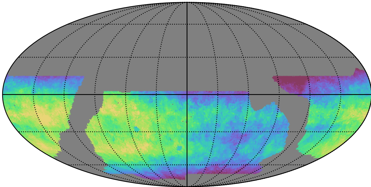
baseline_v2.1_10yrs WFD r band: Median saturation_mag
