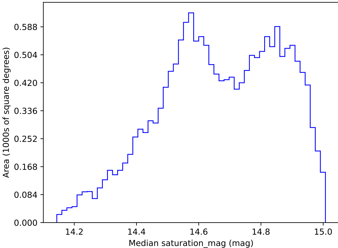
baseline_v2.1_10yrs WFD r band: Median saturation_mag
