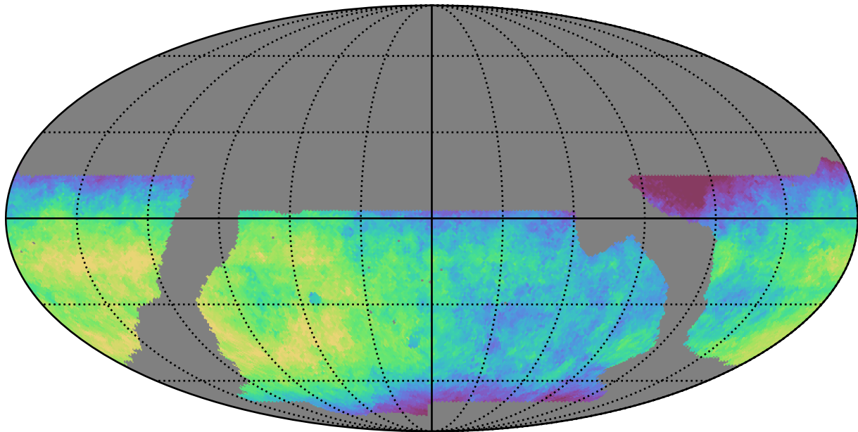
baseline_v2.1_10yrs WFD i band: Median saturation_mag
