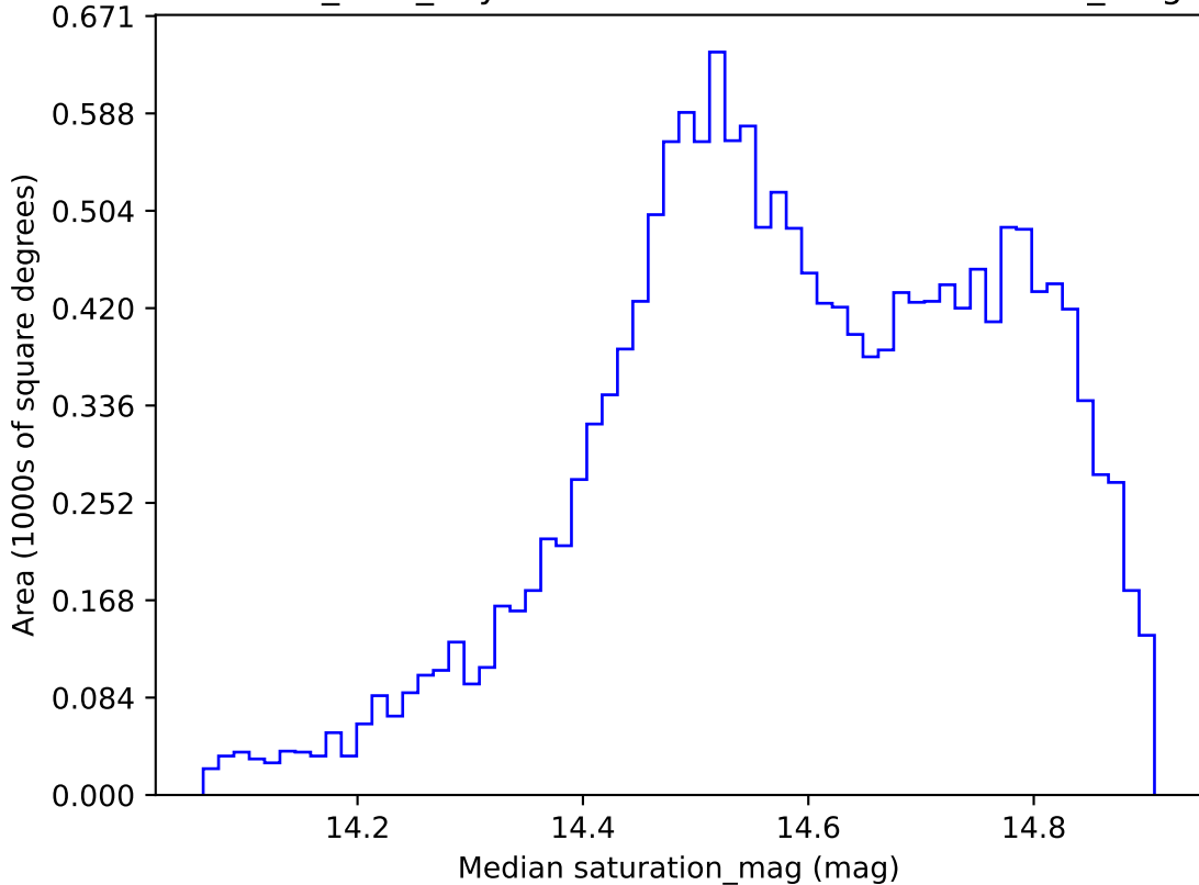
baseline_v2.1_10yrs WFD i band: Median saturation_mag
