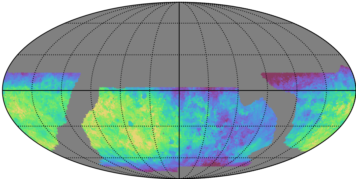
baseline_v2.1_10yrs WFD g band: Median saturation_mag
