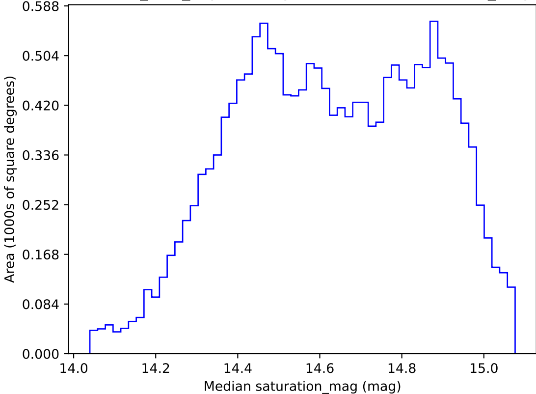
baseline_v2.1_10yrs WFD g band: Median saturation_mag
