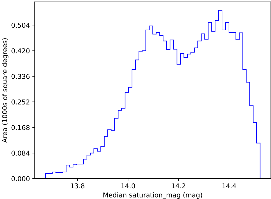
baseline_v2.1_10yrs WFD all bands: Median saturation_mag
