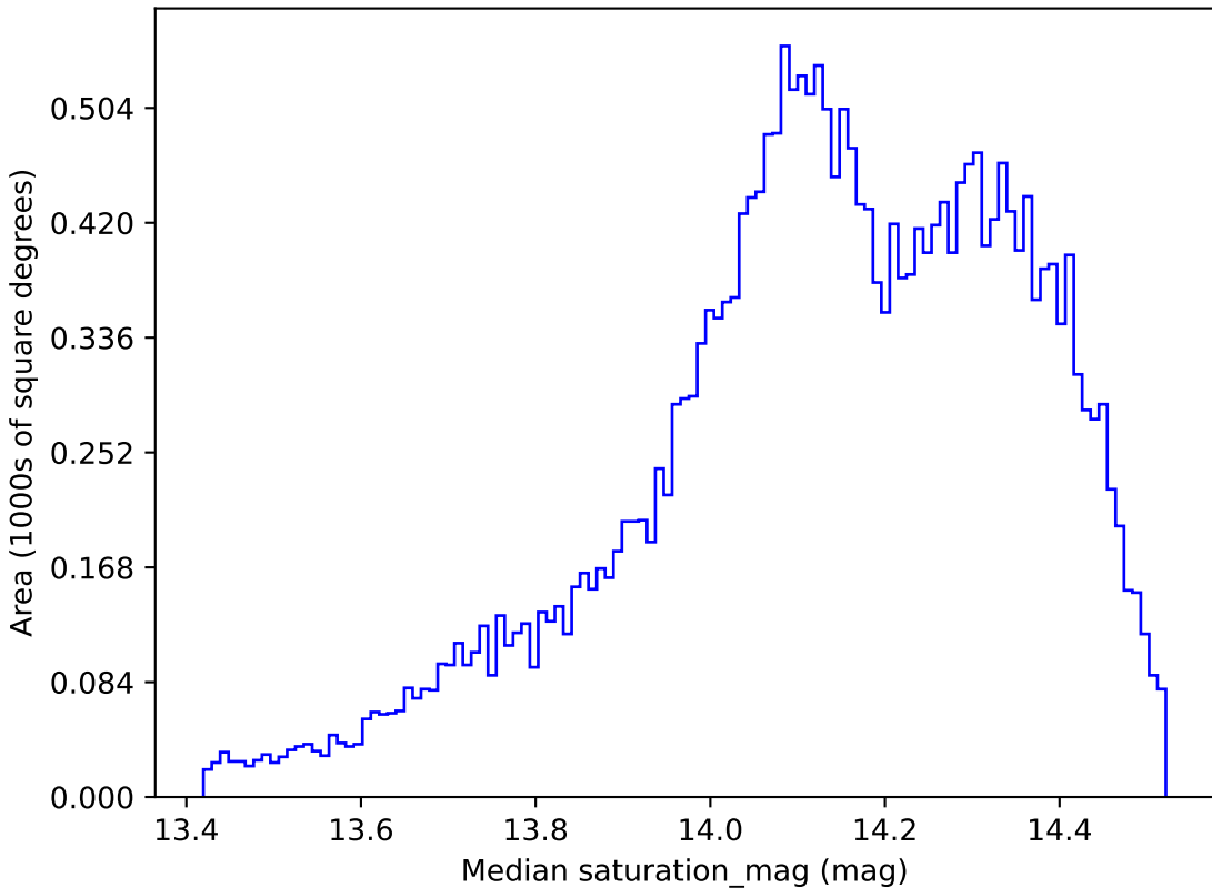
baseline_v2.1_10yrs All sky z band: Median saturation_mag
