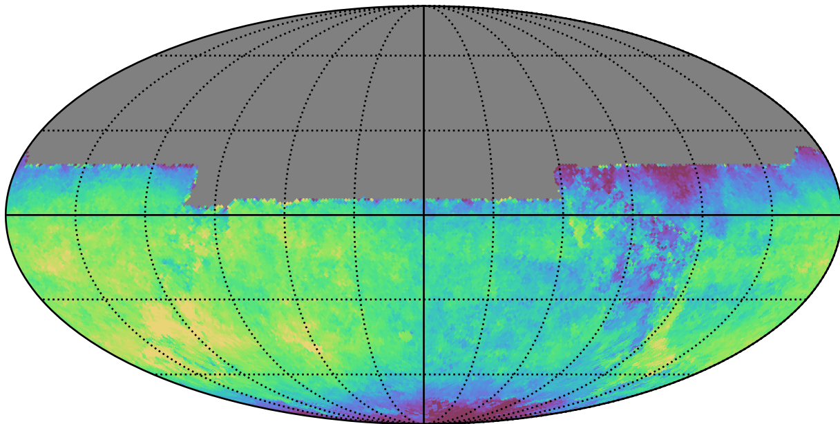
baseline_v2.1_10yrs All sky y band: Median saturation_mag
