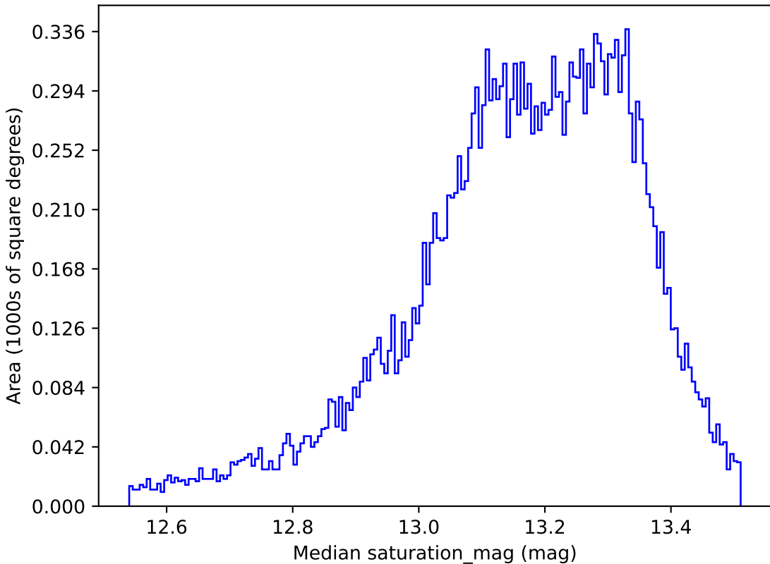
baseline_v2.1_10yrs All sky y band: Median saturation_mag
