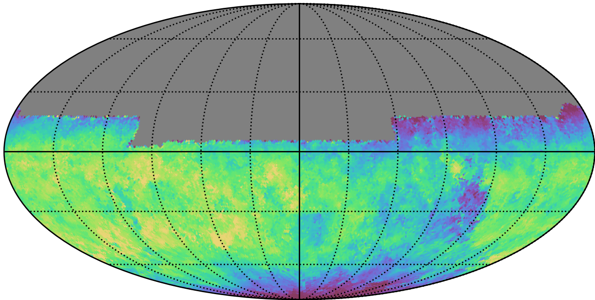
baseline_v2.1_10yrs All sky u band: Median saturation_mag
