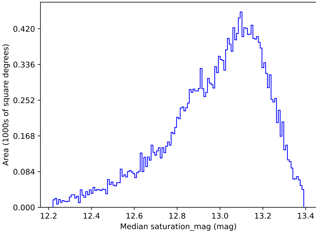
baseline_v2.1_10yrs All sky u band: Median saturation_mag
