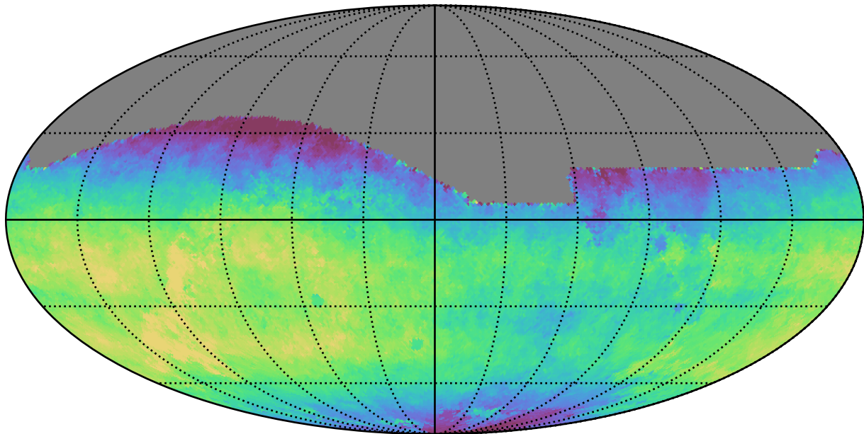
baseline_v2.1_10yrs All sky r band: Median saturation_mag
