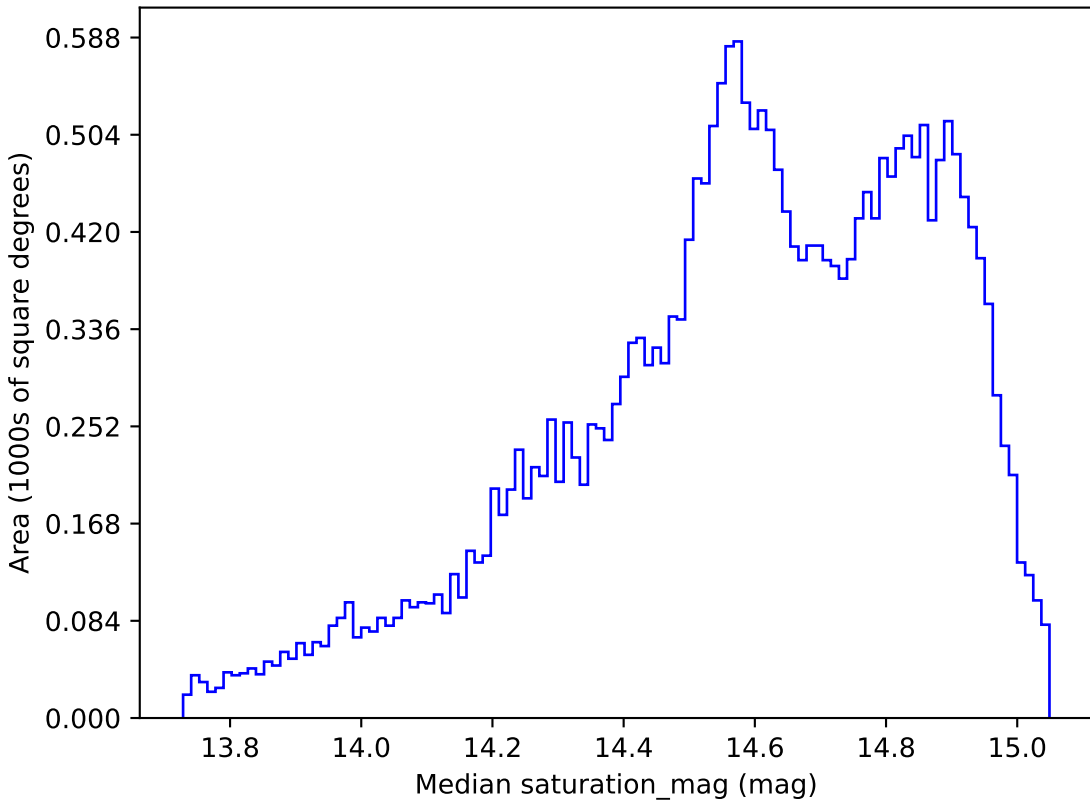
baseline_v2.1_10yrs All sky r band: Median saturation_mag
