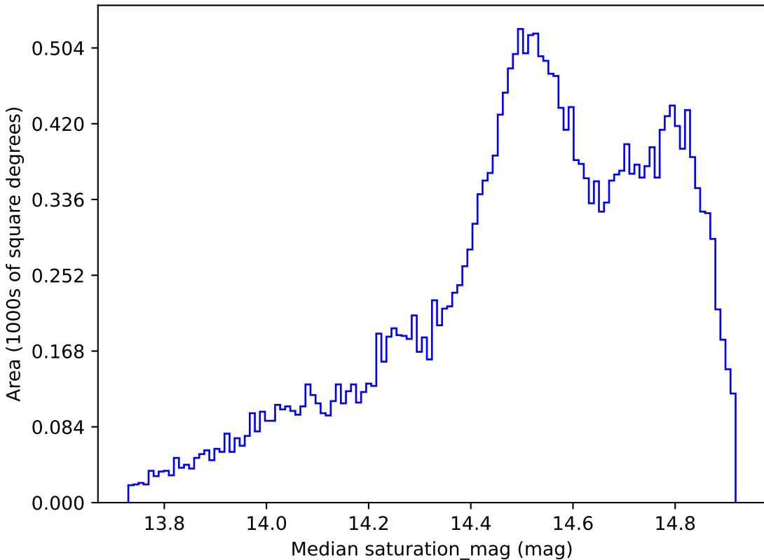
baseline_v2.1_10yrs All sky i band: Median saturation_mag
