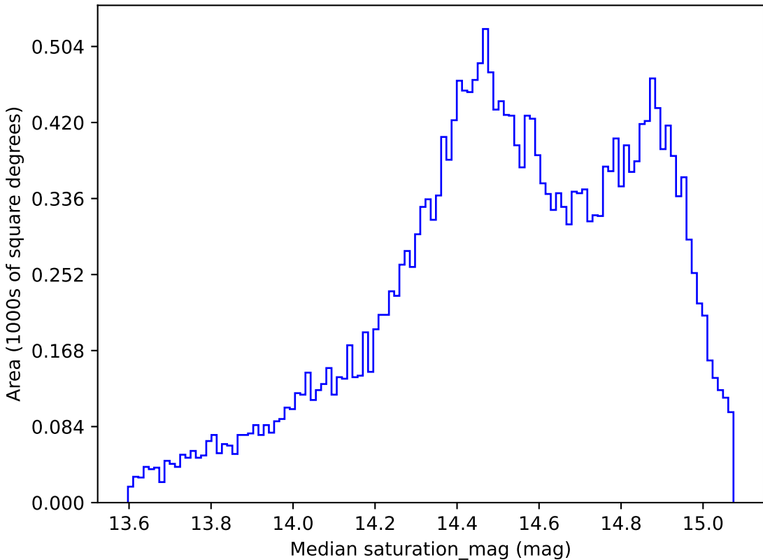
baseline_v2.1_10yrs All sky g band: Median saturation_mag
