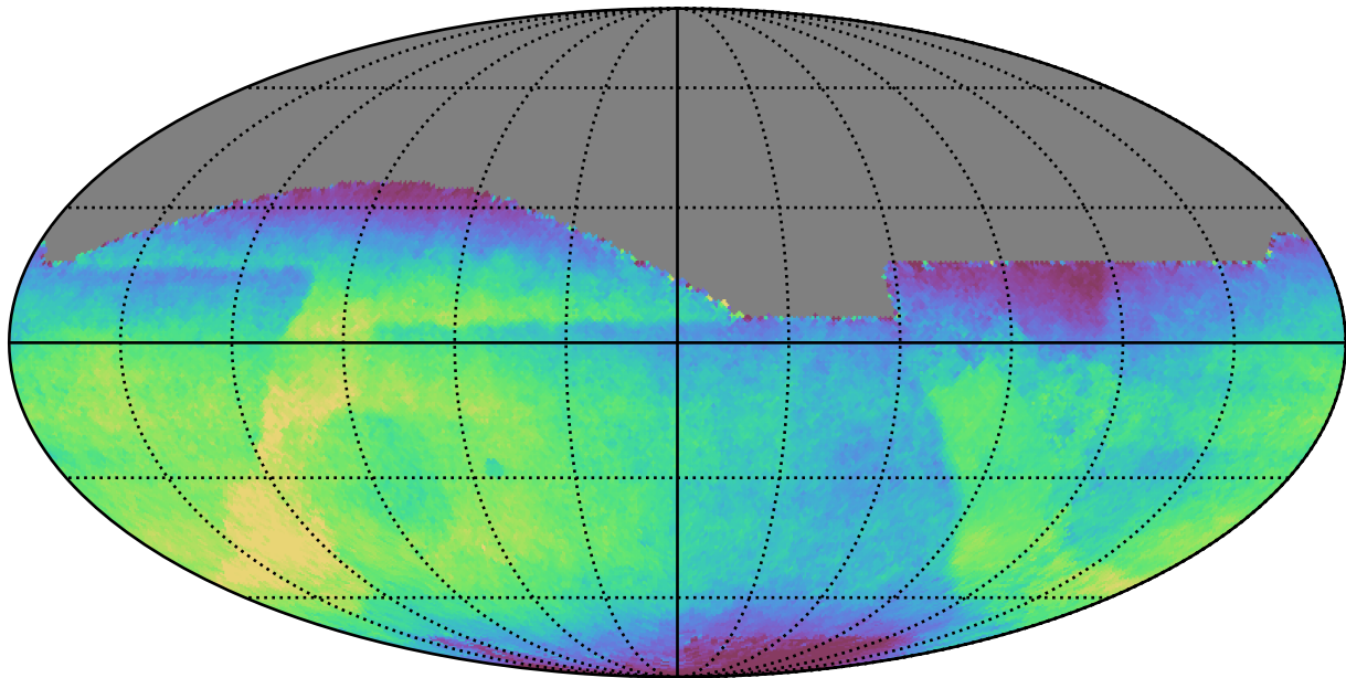
baseline_v2.1_10yrs All sky all bands: Median saturation_mag
