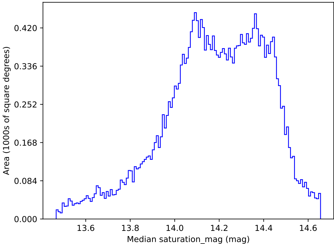
baseline_v2.1_10yrs All sky all bands: Median saturation_mag
