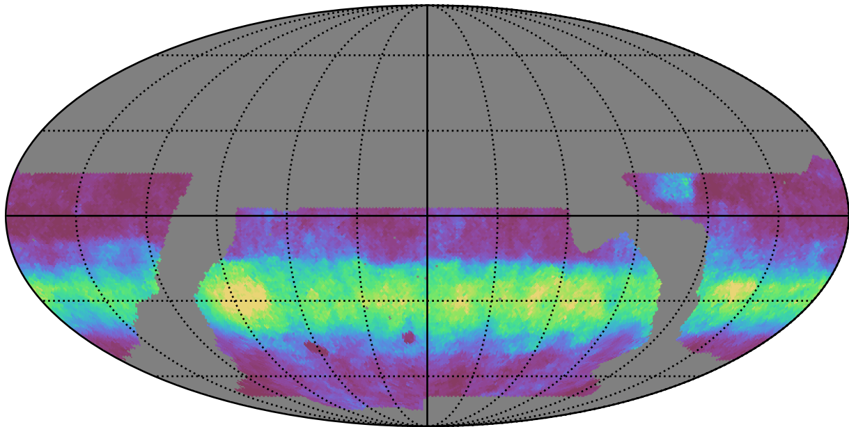
baseline_v2.1_10yrs WFD z band: Median normairmass
