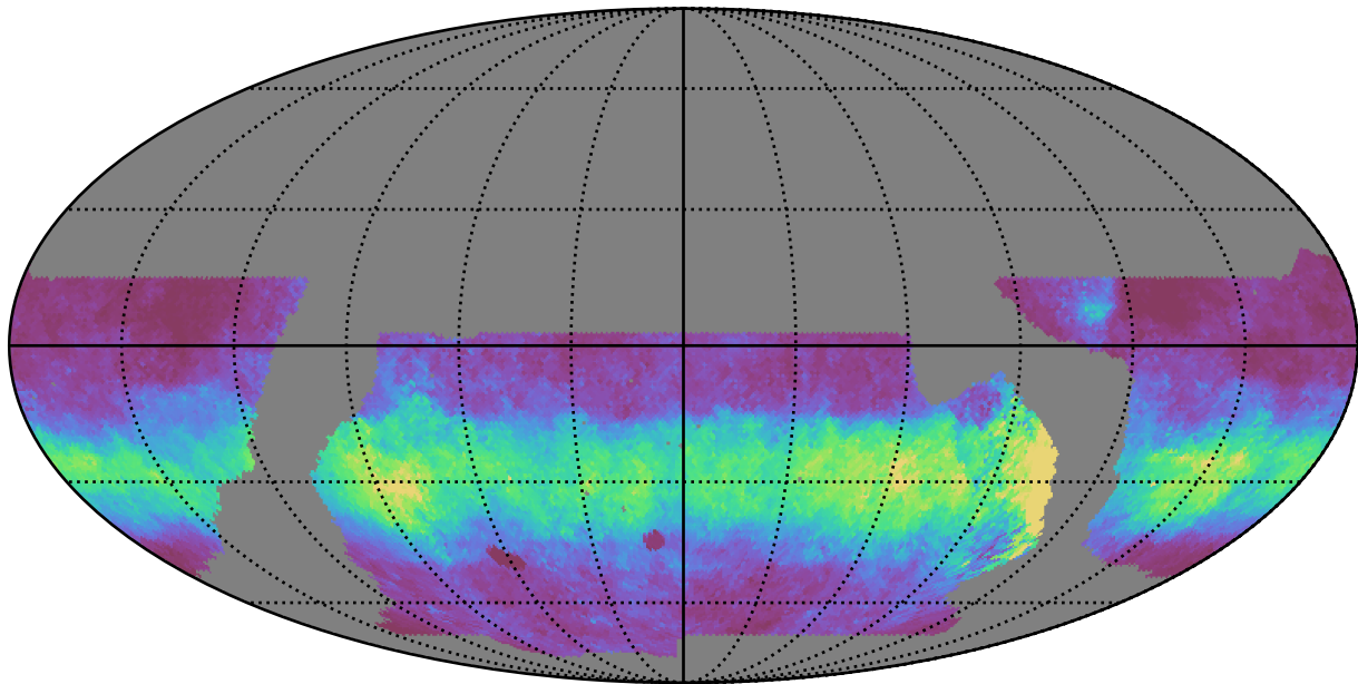
baseline_v2.1_10yrs WFD y band: Median normairmass
