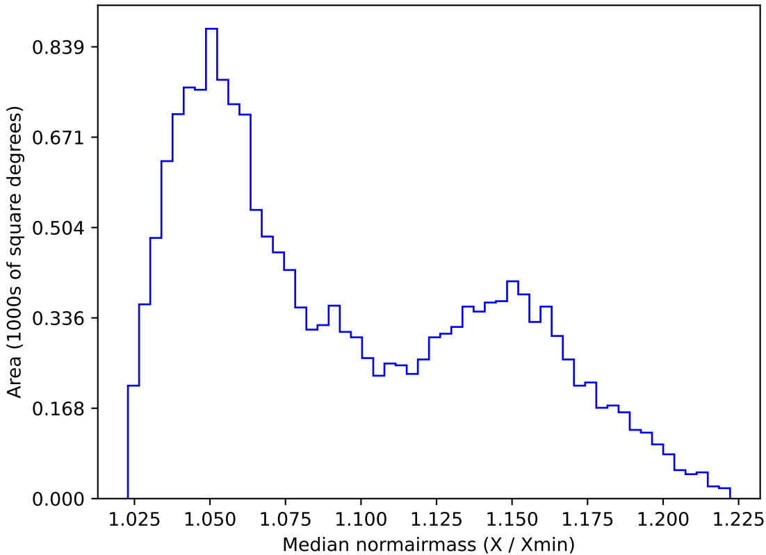
baseline_v2.1_10yrs WFD y band: Median normairmass
